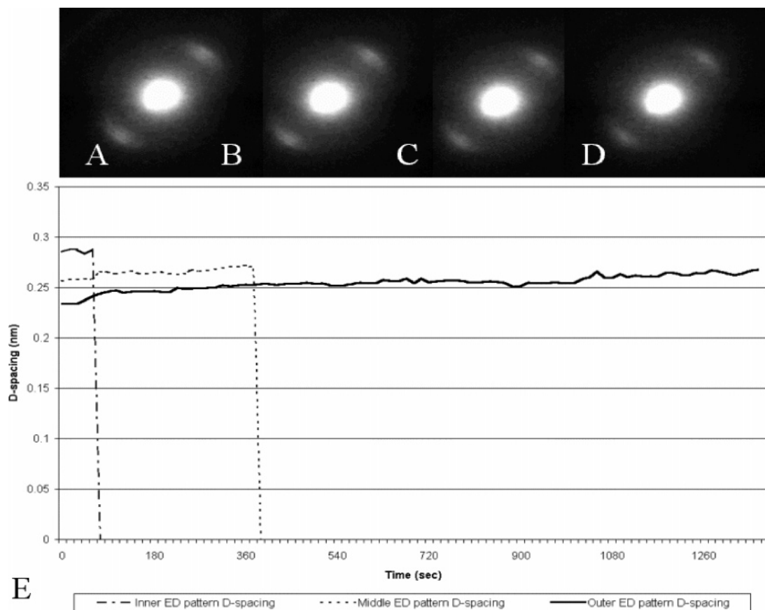
Figure 1. ED time/course analysis of UDPE d-spacings during electron irradiation. (A–D) Draw axis oriented from lower right to upper left. Equatorial reflections are shown. (A) Initial irradiation (beam spot size 6, magnification = 7.5K, accelerating voltage = 100 kV, with a beam current = 0.0025 nA, 230.7 e/Å 2 /s). Note three distinct ED patterns, corresponding to d-spacings 0.2854, 0.2563, and 0.2337 nm. These d-spacings correspond with one-half of the dimensions of the 010 unit cell axis. (B) 90 s irradiation. Total irradiation is approximately 20 763 e/Å 2 . (C) 405 s irradiation. Total irradiation is approximately 93 433 e/Å 2 . (D) 600 s irradiation. Total irradiation is approximately 138 420 e/Å 2 . (E) Graph of the d-spacings vs time.
